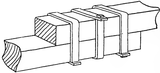
LAPPED & STRAPPED
